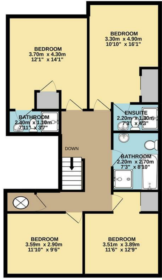
1ST FLOOR
